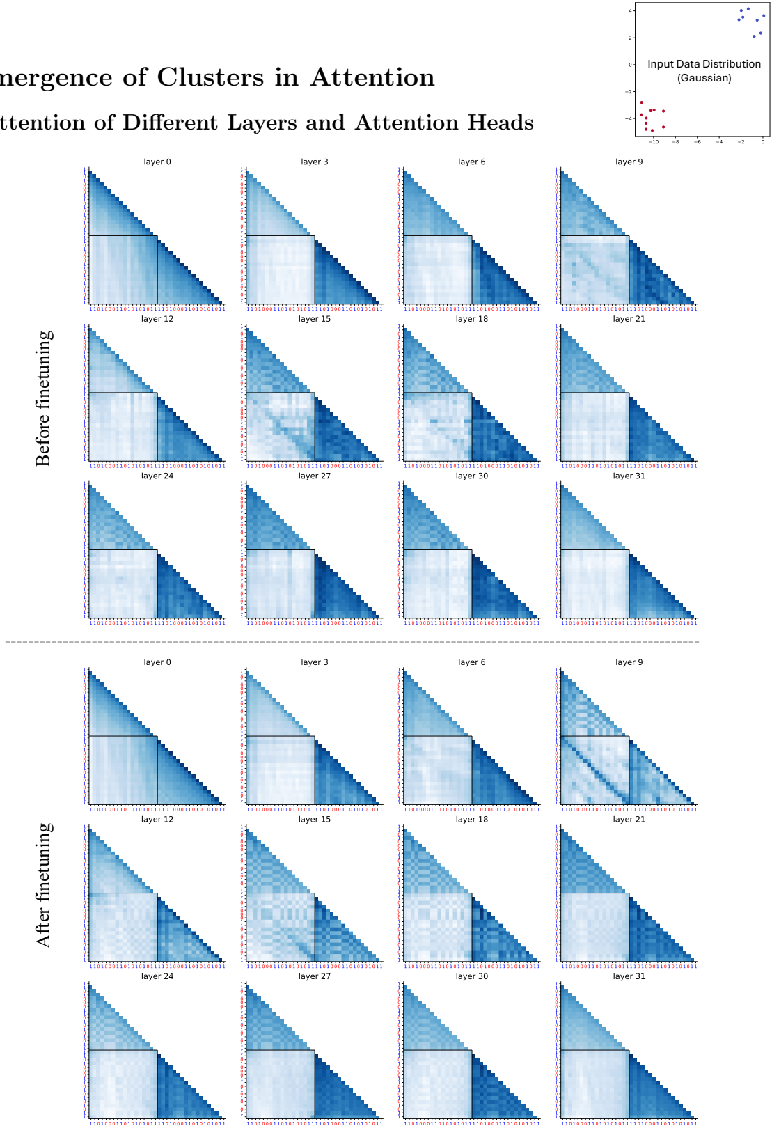
Figure 8: Attention Allocation of LLAMA-3.1-8B-INSTRUCT across Layers. The attention scores are logarithmized for better visualization. Each cluster is generated from a Gaussian distribution, as shown in top right. Figure 3 is a zoom-in view of layer 15 here.
