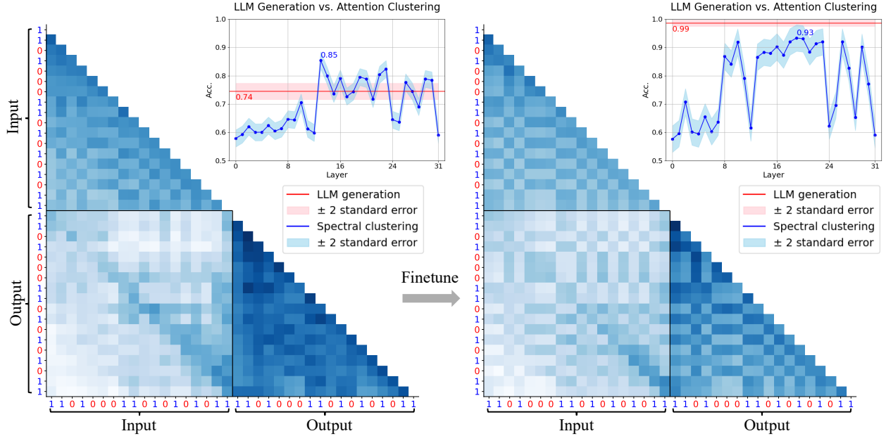
Figure 3: Visualization of Attention Allocation of Input Data and Generated Cluster Labels at an Intermediate Layer. The x-axis and y-axis are the ground-truth cluster labels. The left figure is for the pretrained LLAMA-3.1-8B-INSTRUCT, and the right is after fine-tuning(details in Section 4.1). The top right curves are the average accuracy of spectral clustering using the input-input attention score matrices (top-left) across different layers, compared with the average accuracy of LLM generation.
