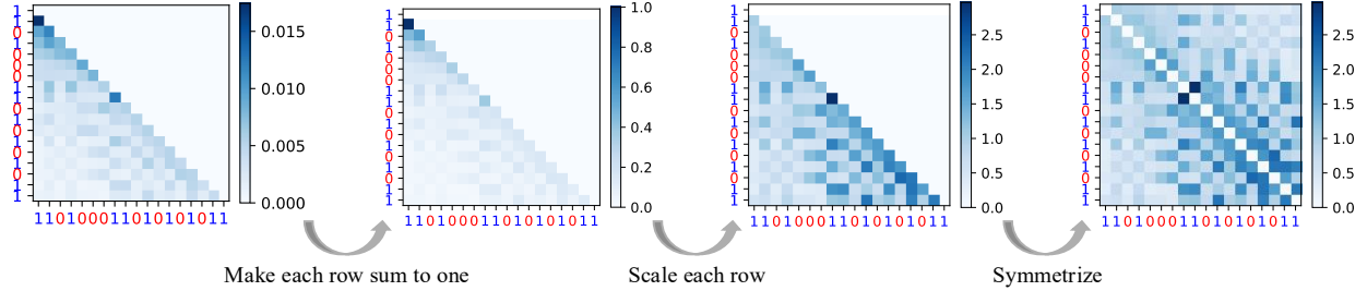
Figure 11: Preprocessing Attention Matrix for Spectral Clustering.
