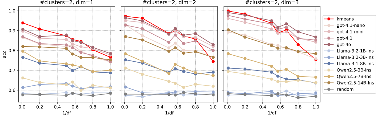
Figure 2: Zero-shot Clustering Accuracy on t -Distribution with Different Degrees of Freedom. When df is small, the data distribution has a heavy tail, which violates the Gaussian assumption of k-means. LLMs show impressive zero-shot clustering capabilities on heavy-tailed data.
