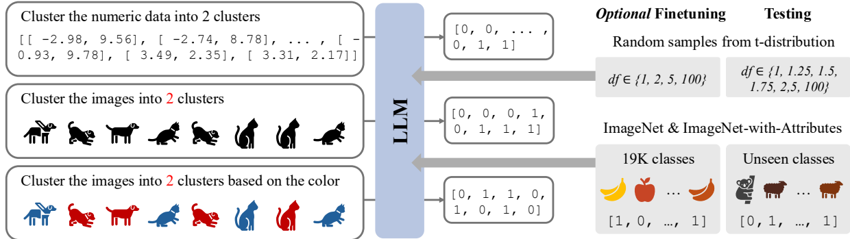
Figure 1: In-Context Clustering (ICC). LLMs can flexibly handle diverse modalities and perform text-conditioned clustering. We show the zero-shot clustering capability in pretrained LLMs and further strengthen it through finetuning.
