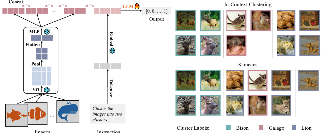
Figure 4: Left: Multimodal LLM Architecture with Average Pooling for Image Features. Right: Qualitative Comparison of Models on Image Clustering — ICC outperforms k-means when the data has rich semantic information.
