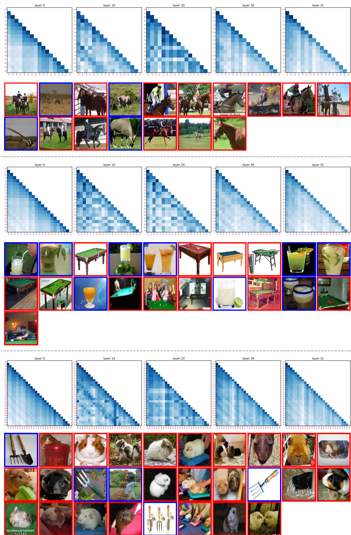
Figure 13: Attention Allocation of Image Clustering. Different colors represent different clusters.
