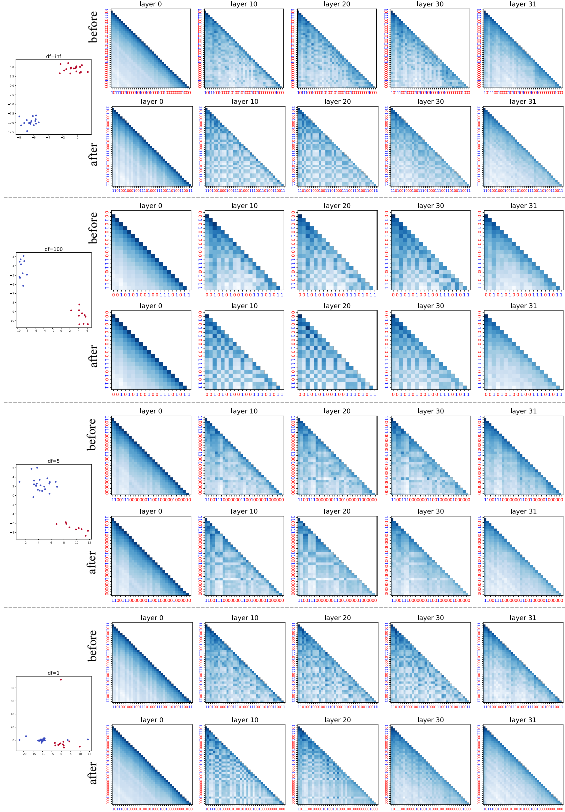
Figure 9: Attention Allocation of LLAMA-3.1-8B-INSTRUCT on t -Distributed Data with Different df , before and after Finetuning. Note that t -distribution with df = inf is Gaussian. The attention scores are logarithmized for better visualization.
